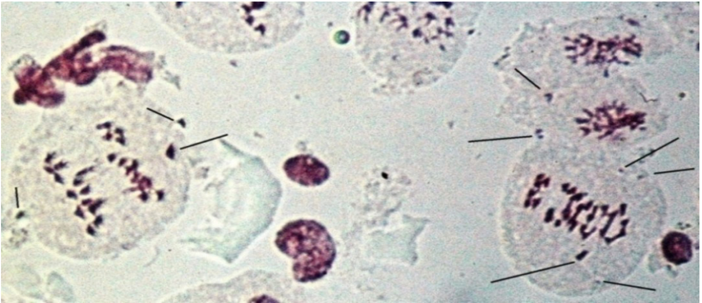
Figure: 3 Meiosis in Isoetes pantii A. A megaspore mother cell at an early anaphase I in a heterosporangium revealed many chromatin dots which appear to have arisen due to fragmentation of chromosomes and also chromatin attenuation of a few chromosomes. The anaphasic separation shows reduced chromosome number, 14 at one and 13 chromosomes moving towards the respective poles (Photographed at 100 x 10) ;
